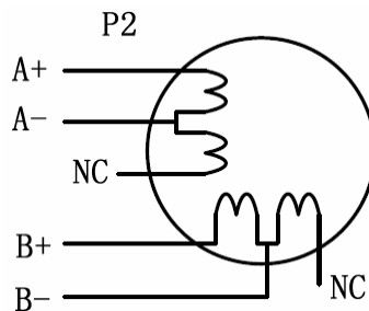
Figure 5-2: 6-lead motor half coil (higher speed) connections
