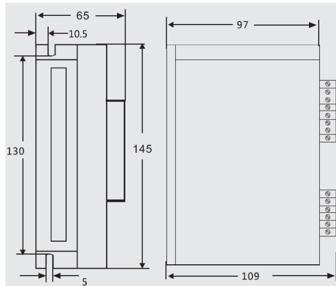
Figure 2-1 Mechanical Specification
