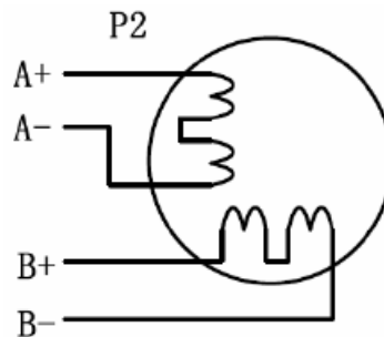
Figure 5-1: 4-lead Motor Connections
