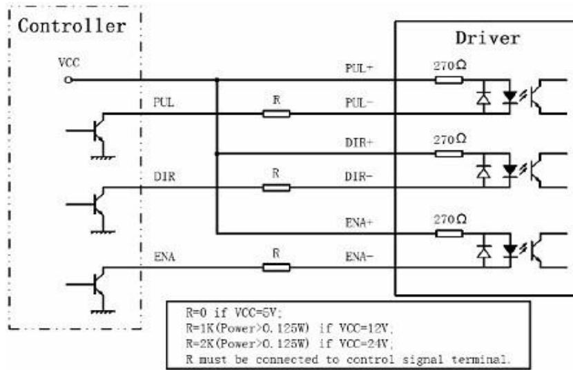
Figure 4-1: Connections to open-collector signal (common-anode)
