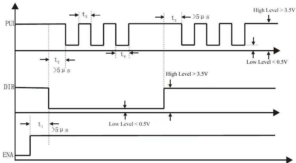
Figure 4-3 Sequence chart of control signals
