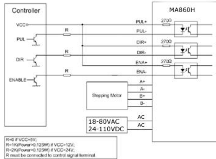
Figure 9-1: Typical connection
