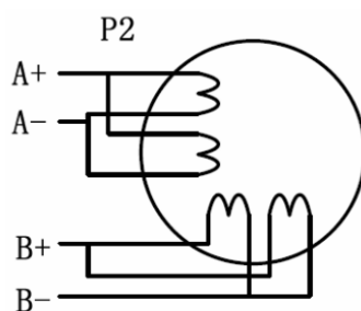
Figure 5-5: 8-lead motor parallel connections
