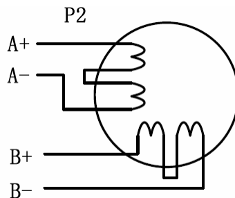
Figure 5-4: 8-lead motor series connections
