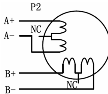
Figure 5-3: 6-lead motor full coil (higher torque) connections
