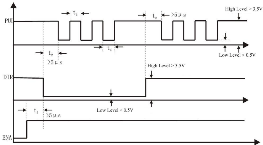
Figure 10-1: Sequence chart of control signals
