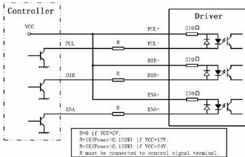
Figure 4-2: Connection to PNP signal (common-cathode)
